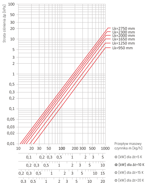
VKN5-7,5/25/Lk, VKN5-9/25/Lk
