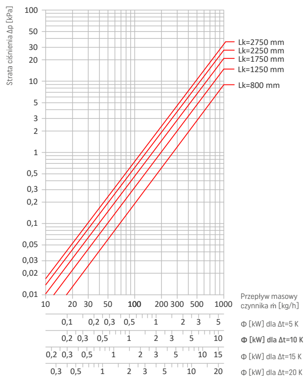
VKN5-14/30/Lk
